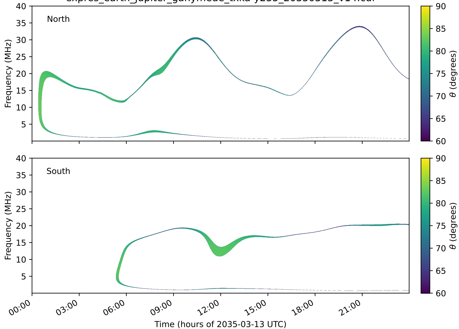
expres_earth_jupiter_ganymede_txka-y235_20350313_v14.cdf
