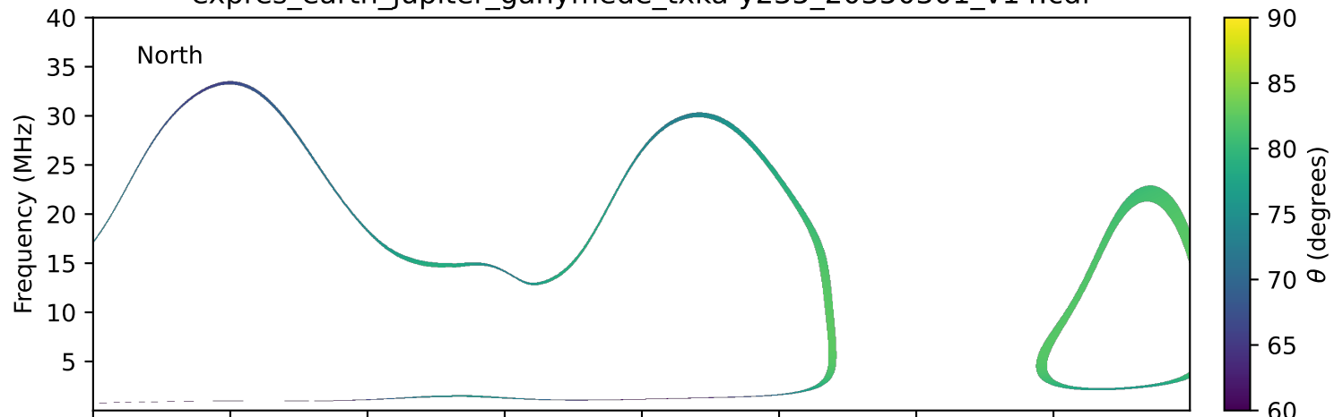
expres_earth_jupiter_ganymede_txka-y235_20350301_v14.cdf
