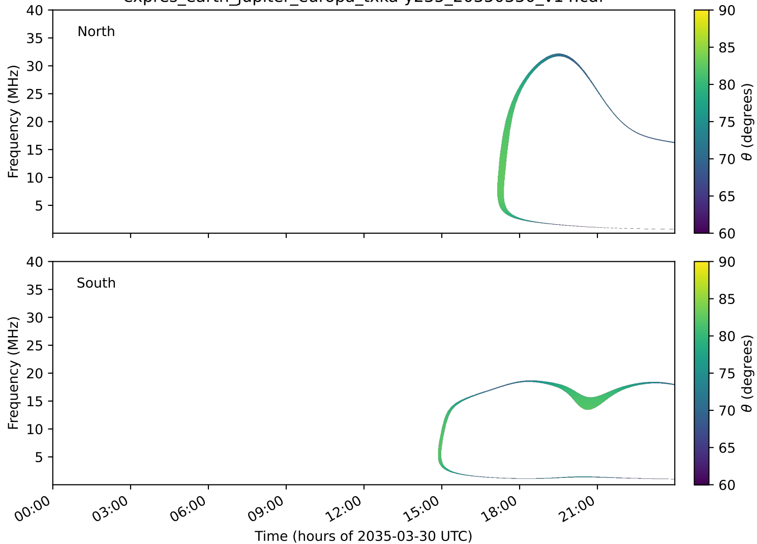
expres_earth_jupiter_europa_txka-y235_20350330_v14.cdf
