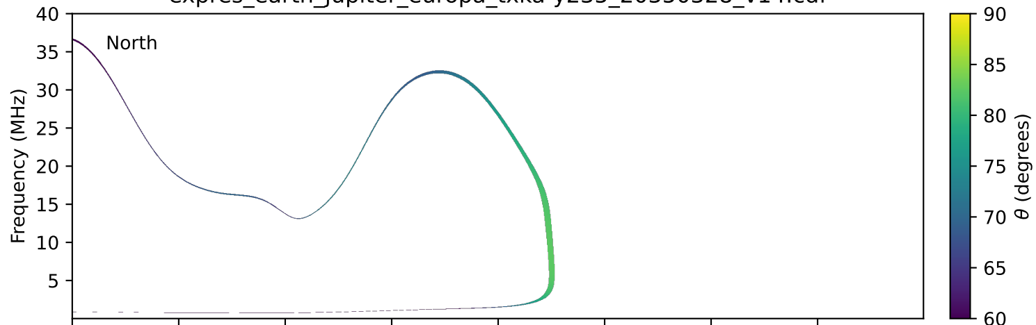
expres_earth_jupiter_europa_txka-y235_20350328_v14.cdf
