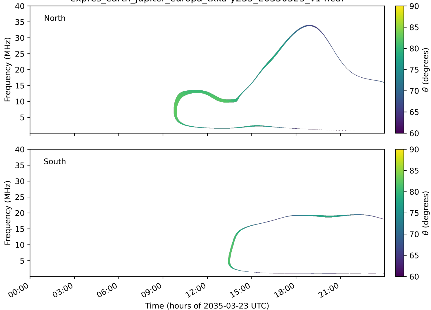
expres_earth_jupiter_europa_txka-y235_20350323_v14.cdf
