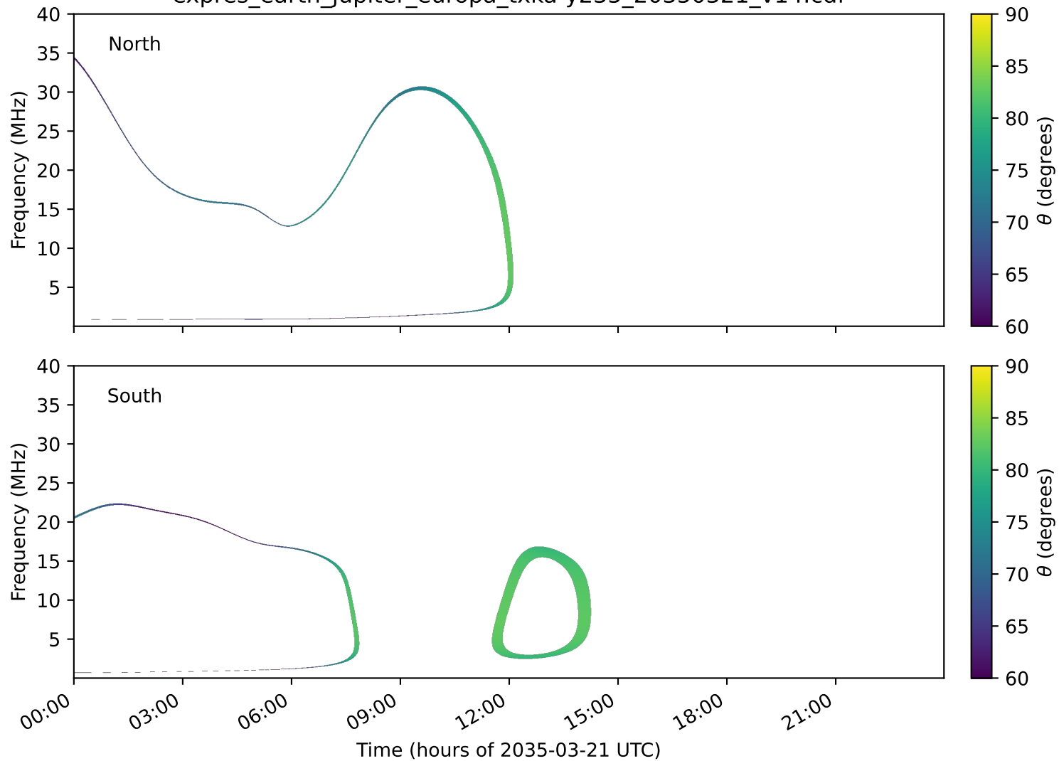
expres_earth_jupiter_europa_txka-y235_20350321_v14.cdf
