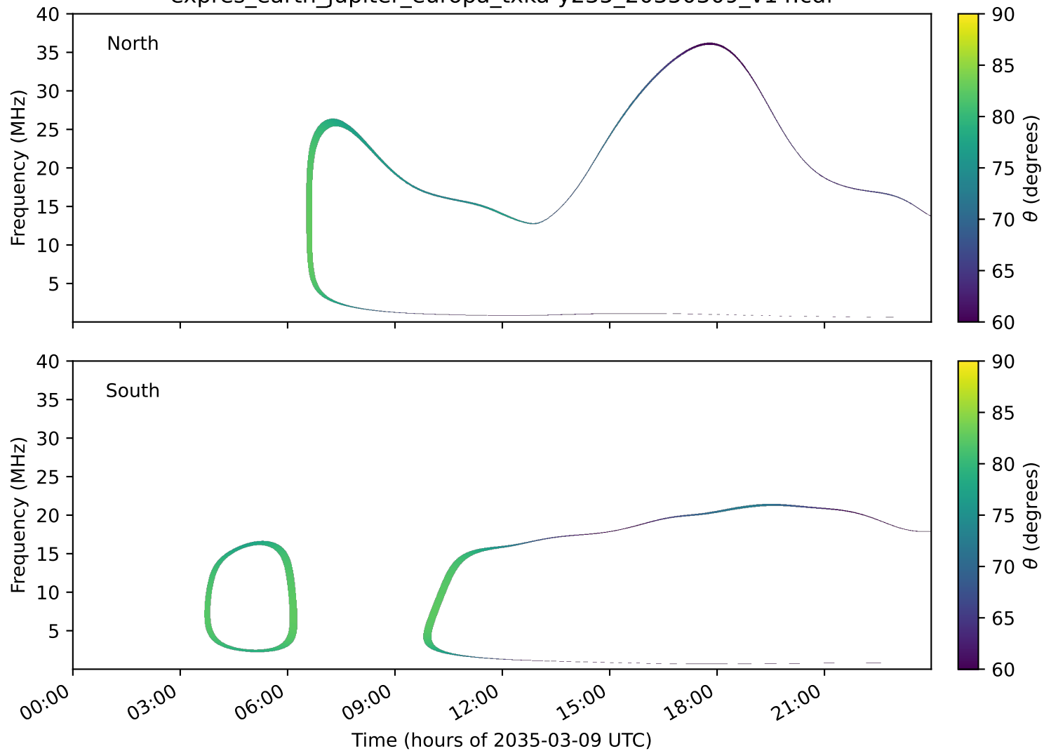
expres_earth_jupiter_europa_txka-y235_20350309_v14.cdf
