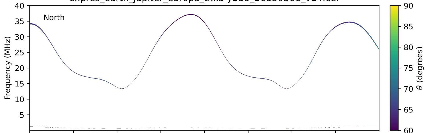
expres_earth_jupiter_europa_txka-y235_20350306_v14.cdf
