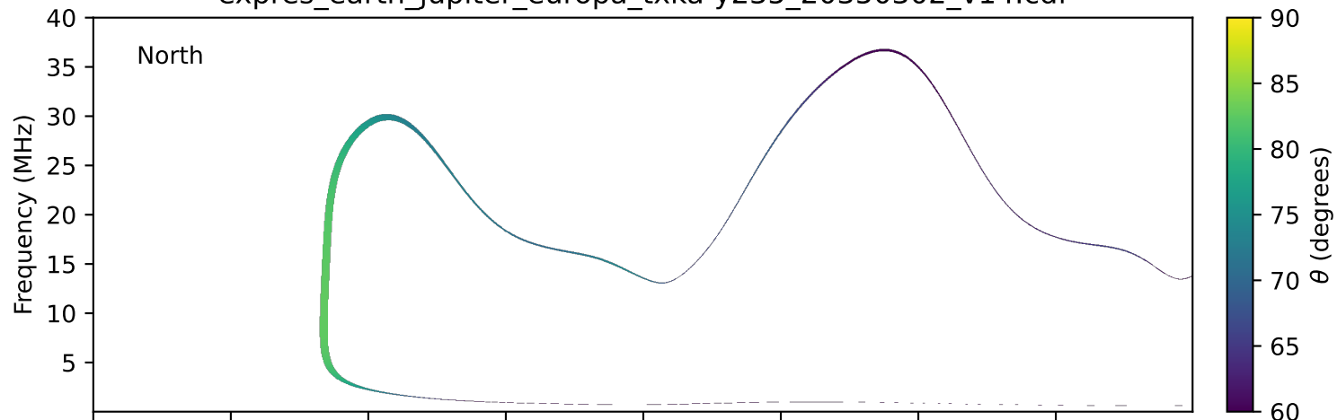
expres_earth_jupiter_europa_txka-y235_20350302_v14.cdf
