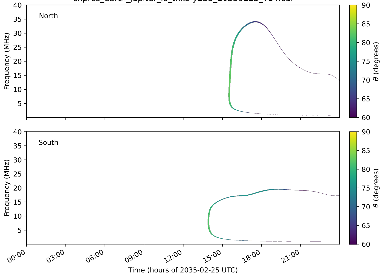
expres_earth_jupiter_io_txka-y235_20350225_v14.cdf
