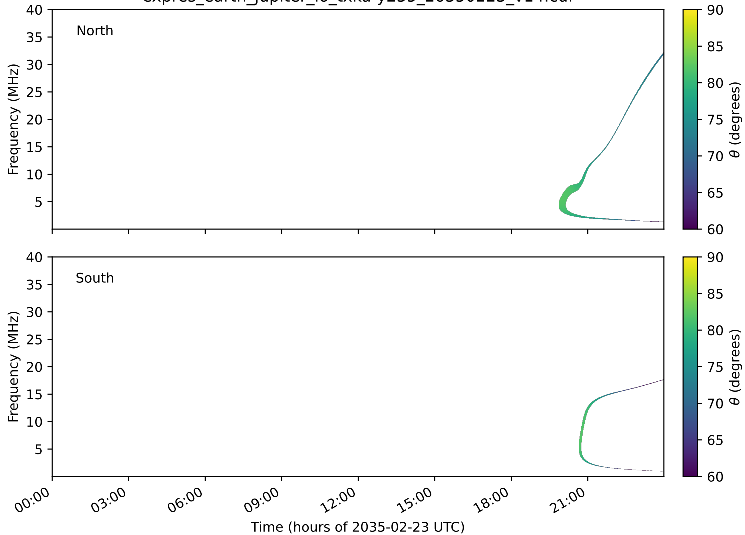
expres_earth_jupiter_io_txka-y235_20350223_v14.cdf
