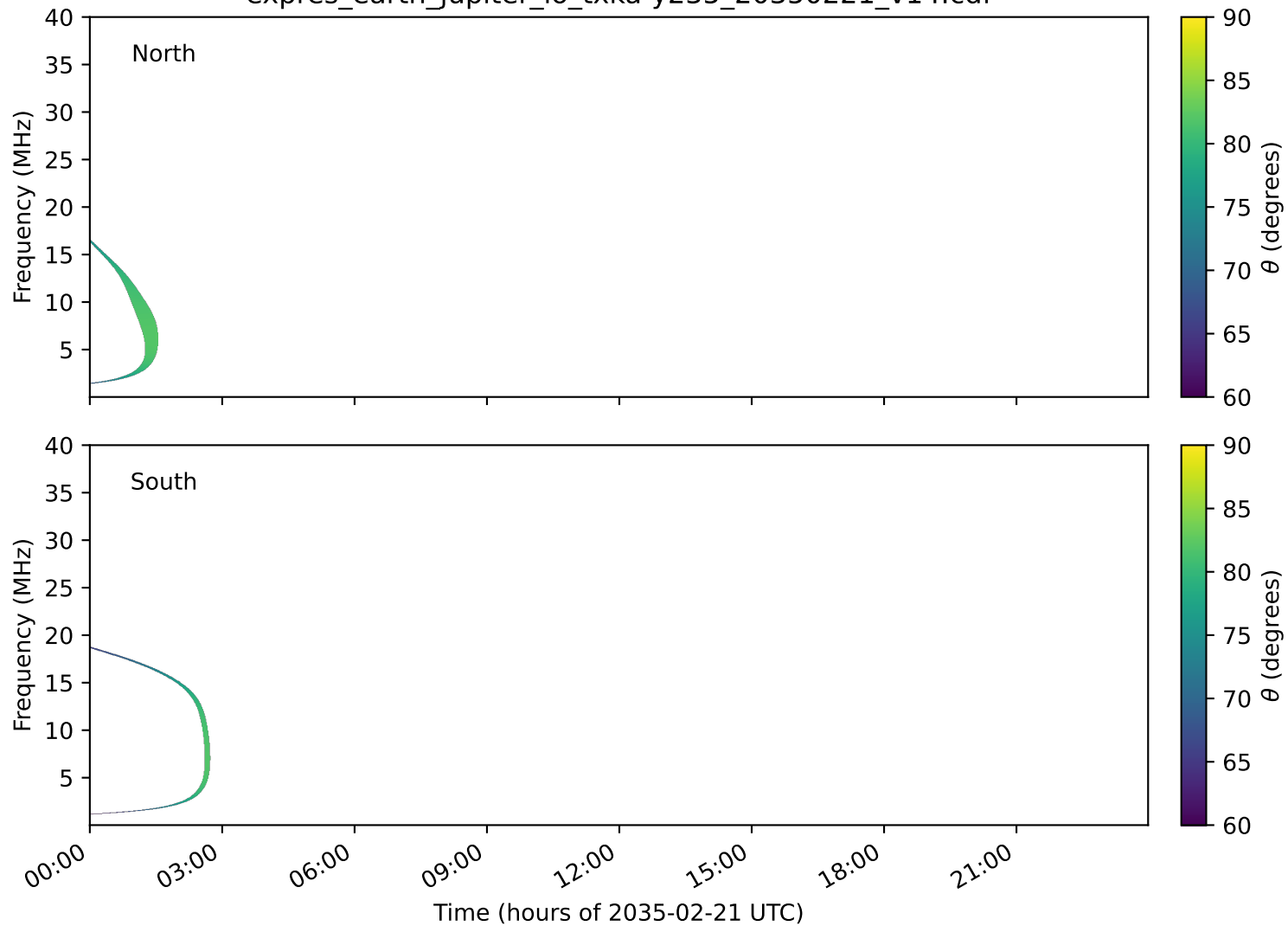
expres_earth_jupiter_io_txka-y235_20350221_v14.cdf
