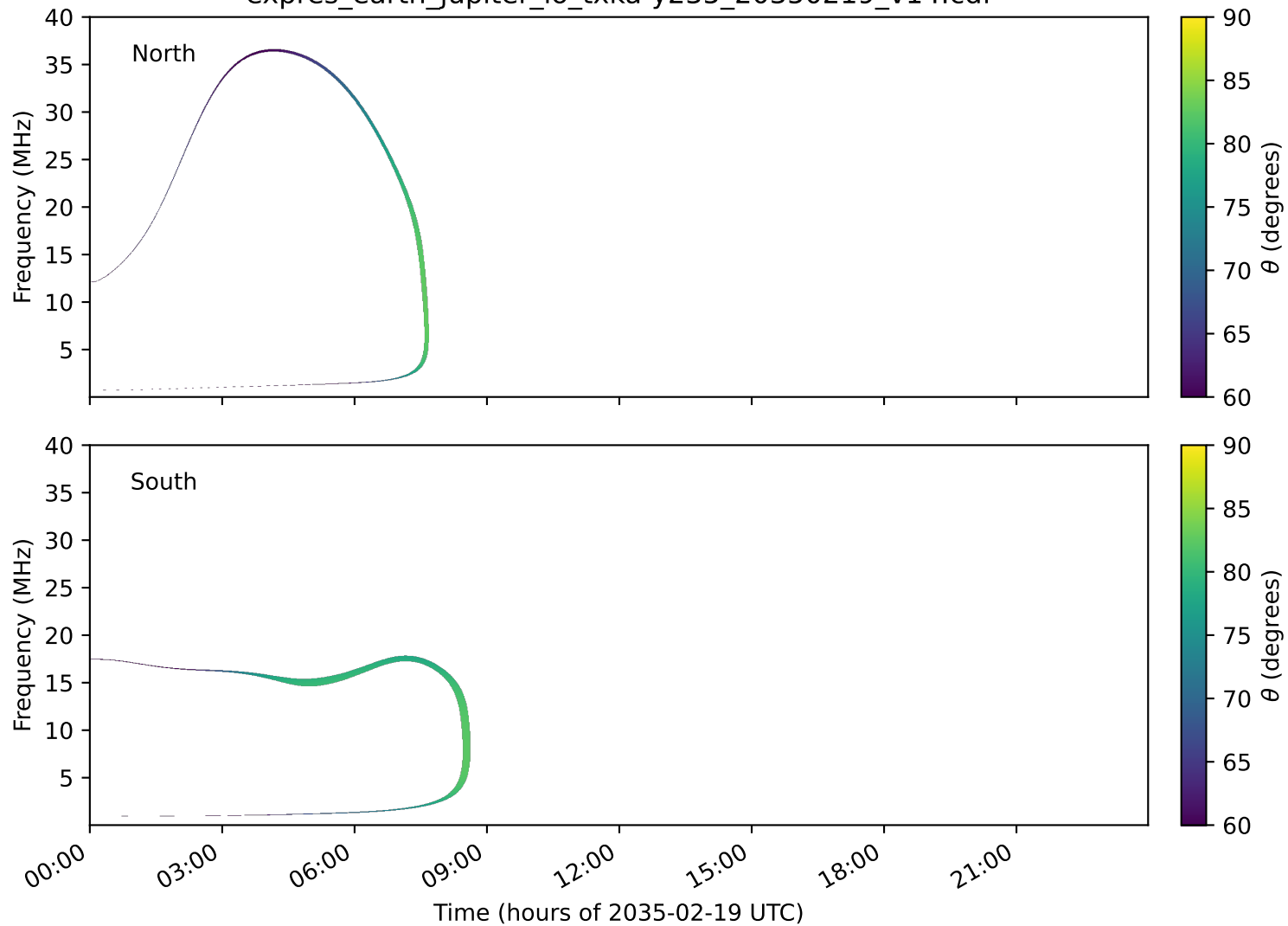
expres_earth_jupiter_io_txka-y235_20350219_v14.cdf
