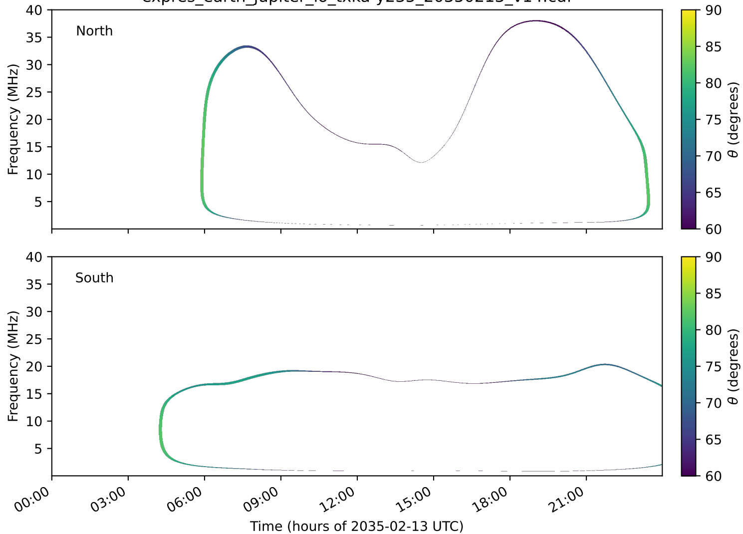
expres_earth_jupiter_io_txka-y235_20350213_v14.cdf
