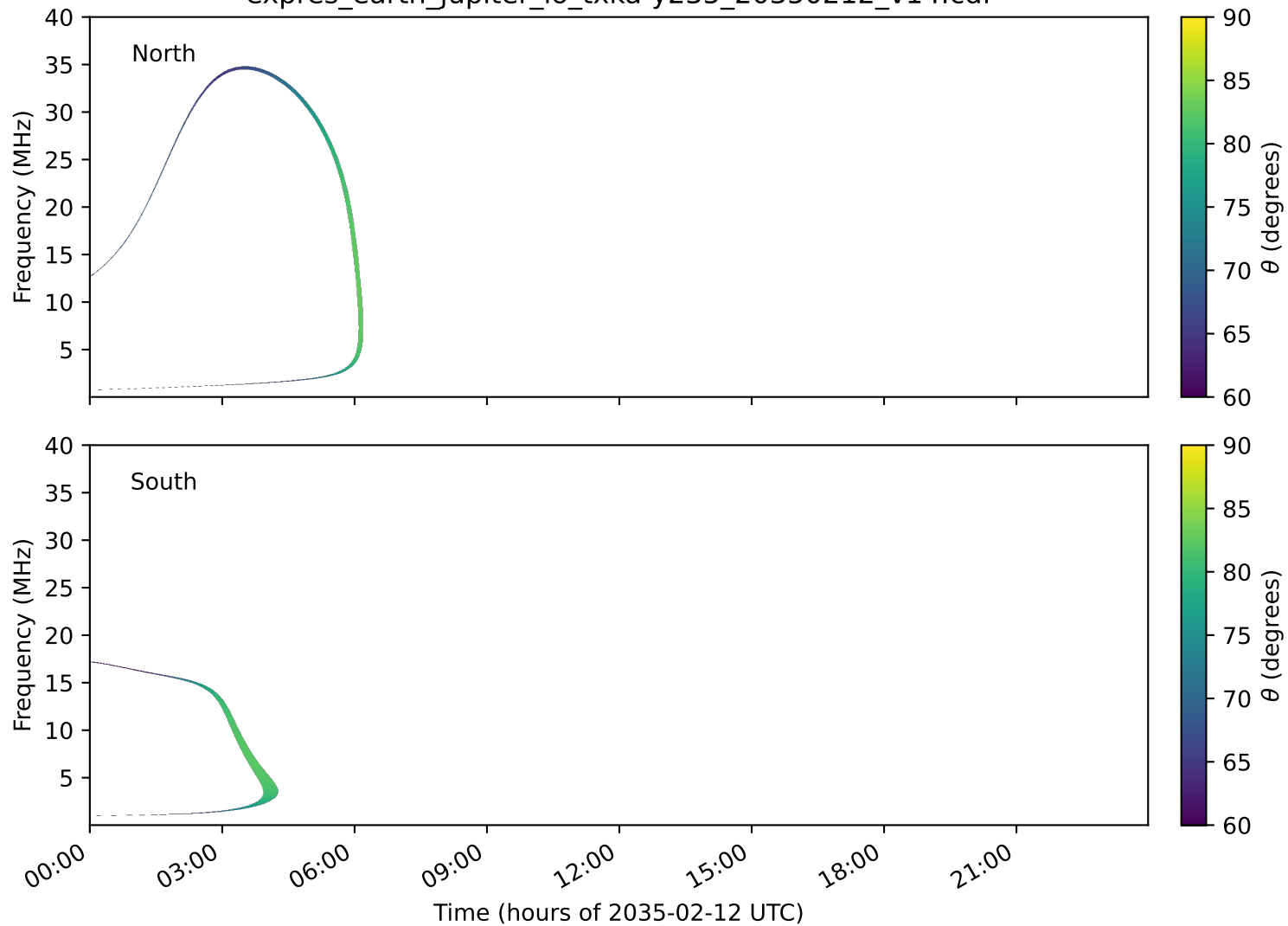
expres_earth_jupiter_io_txka-y235_20350212_v14.cdf
