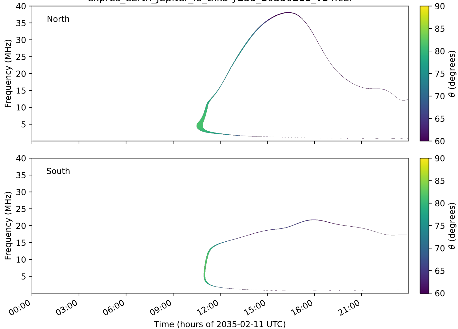
expres_earth_jupiter_io_txka-y235_20350211_v14.cdf
