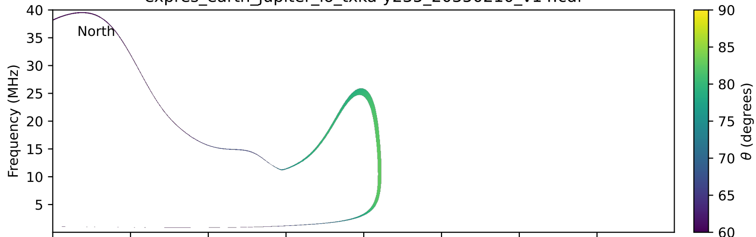
expres_earth_jupiter_io_txka-y235_20350210_v14.cdf
