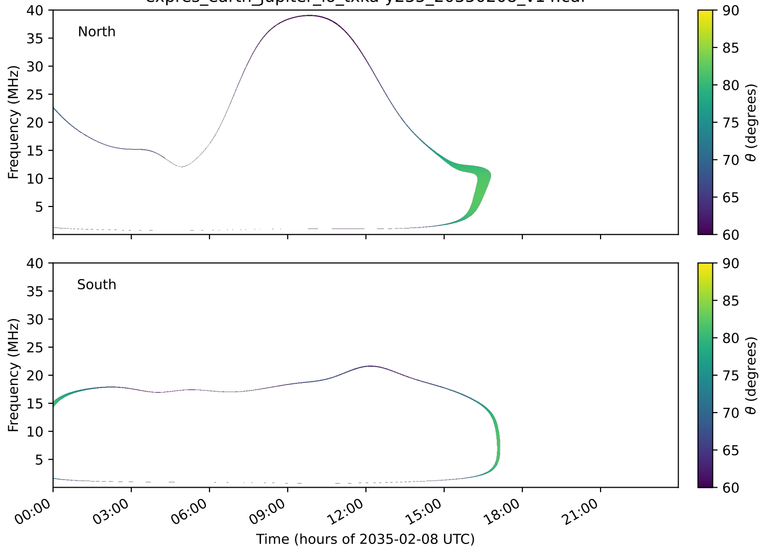
expres_earth_jupiter_io_txka-y235_20350208_v14.cdf
