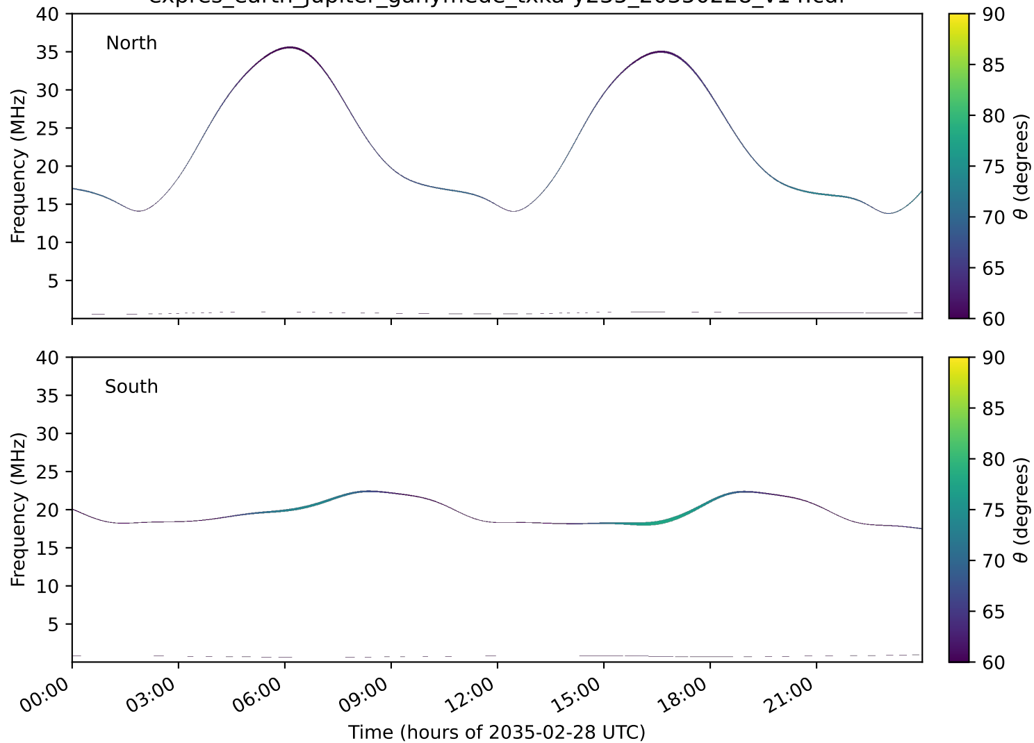
expres_earth_jupiter_ganymede_txka-y235_20350228_v14.cdf
