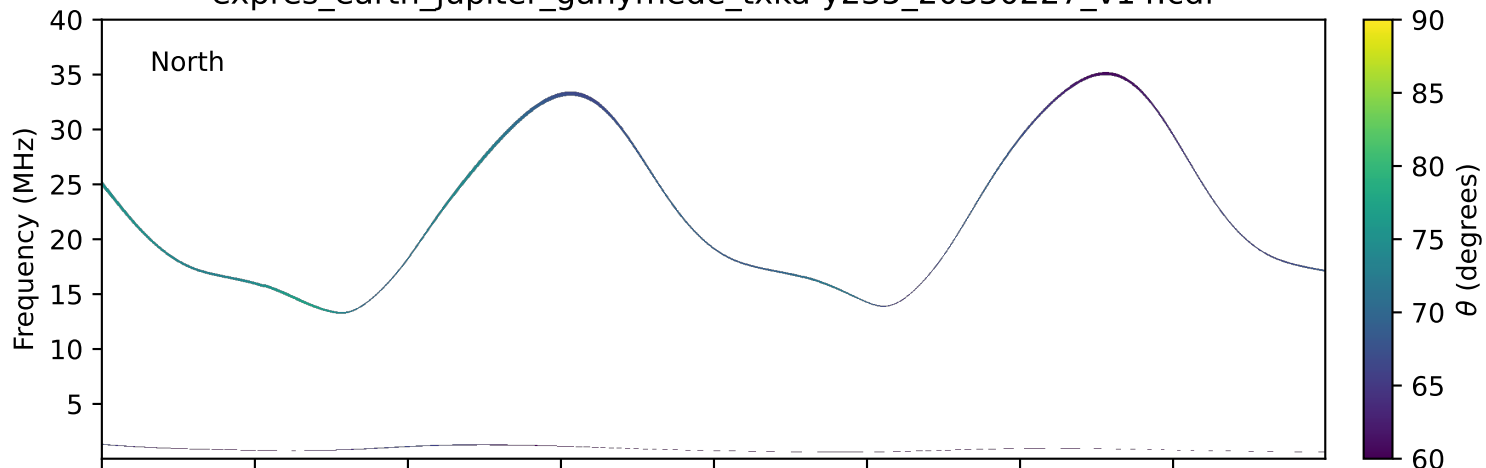
expres_earth_jupiter_ganymede_txka-y235_20350227_v14.cdf
