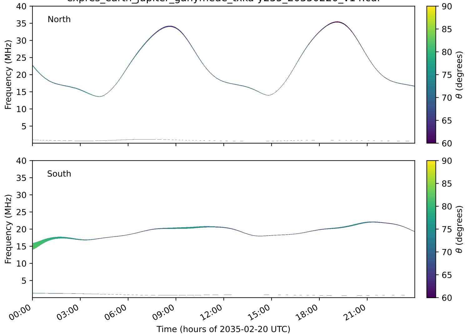
expres_earth_jupiter_ganymede_txka-y235_20350220_v14.cdf
