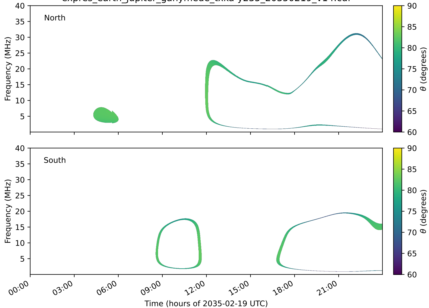
expres_earth_jupiter_ganymede_txka-y235_20350219_v14.cdf
