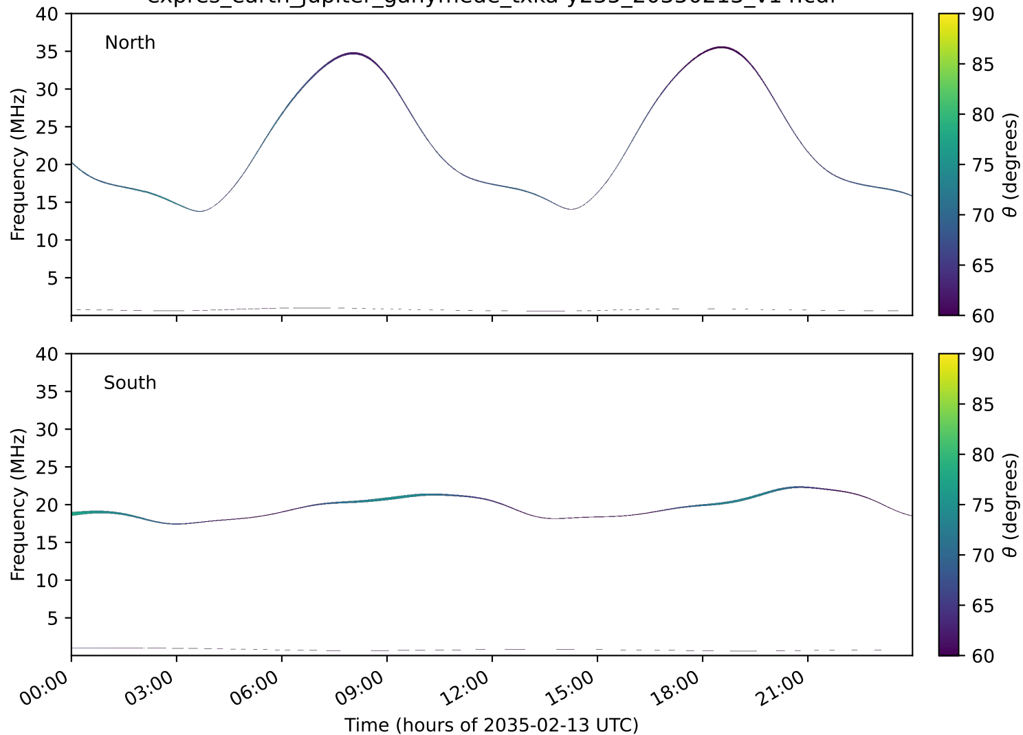
expres_earth_jupiter_ganymede_txka-y235_20350213_v14.cdf
