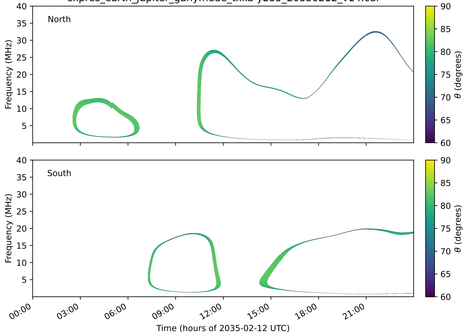
expres_earth_jupiter_ganymede_txka-y235_20350212_v14.cdf
