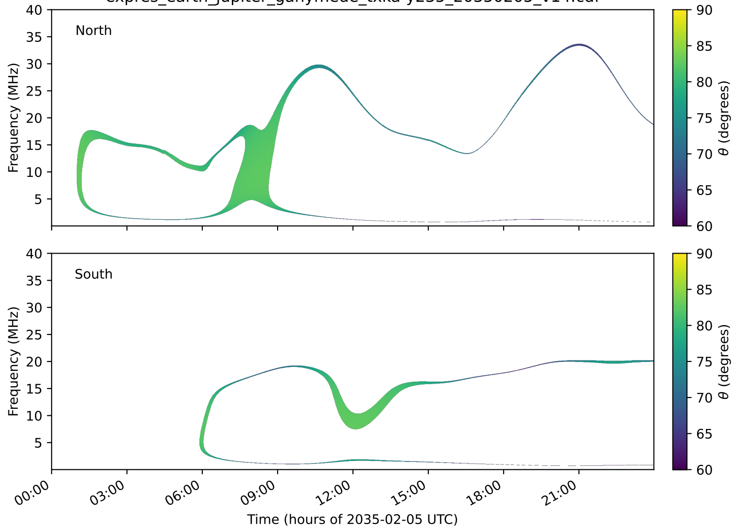
expres_earth_jupiter_ganymede_txka-y235_20350205_v14.cdf
