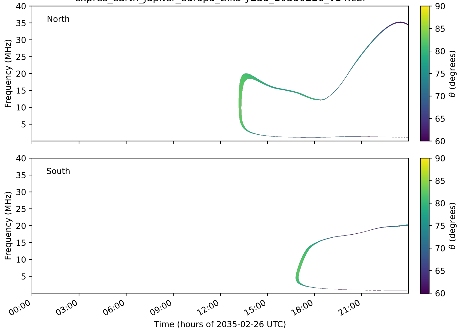
expres_earth_jupiter_europa_txka-y235_20350226_v14.cdf
