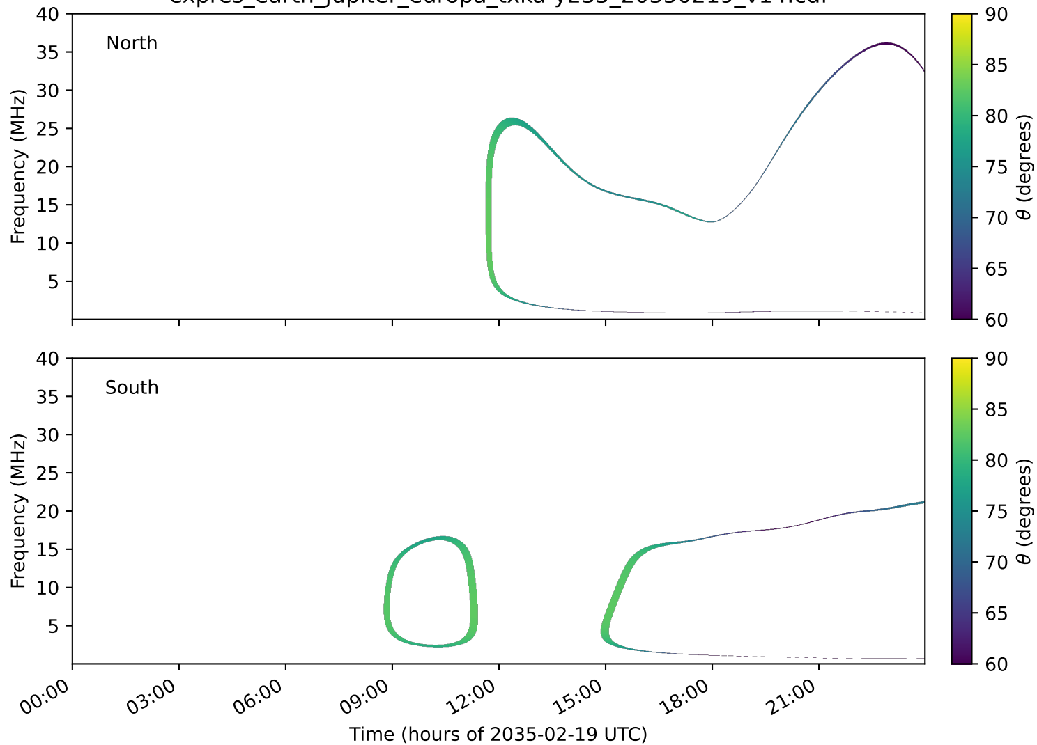
expres_earth_jupiter_europa_txka-y235_20350219_v14.cdf
