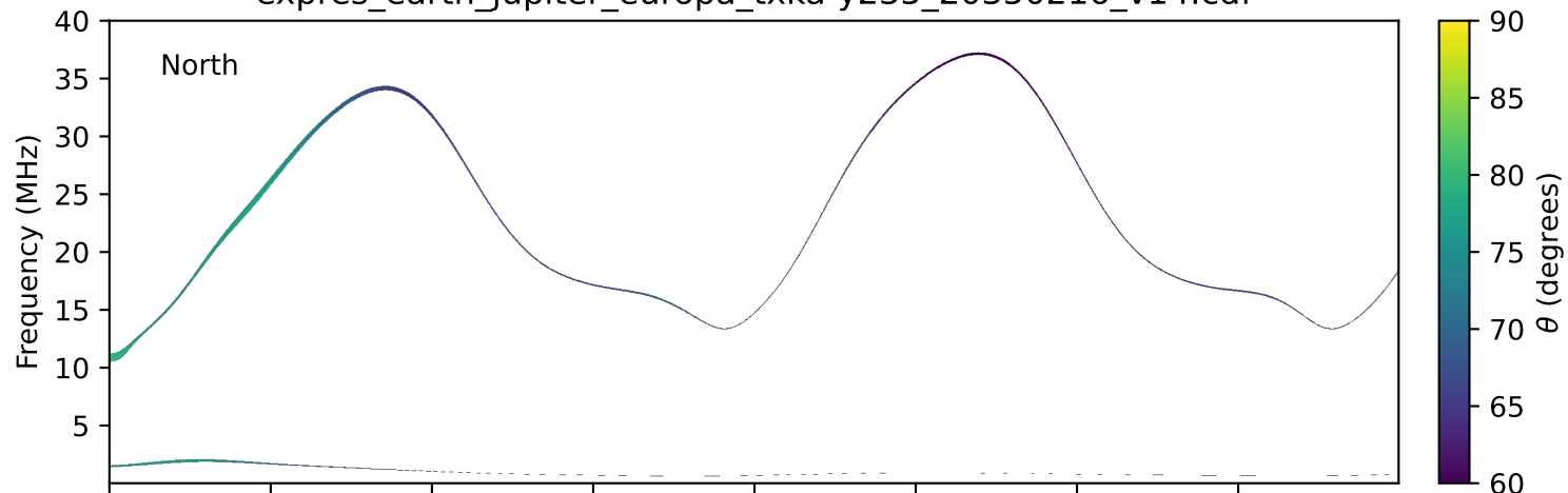
expres_earth_jupiter_europa_txka-y235_20350216_v14.cdf
