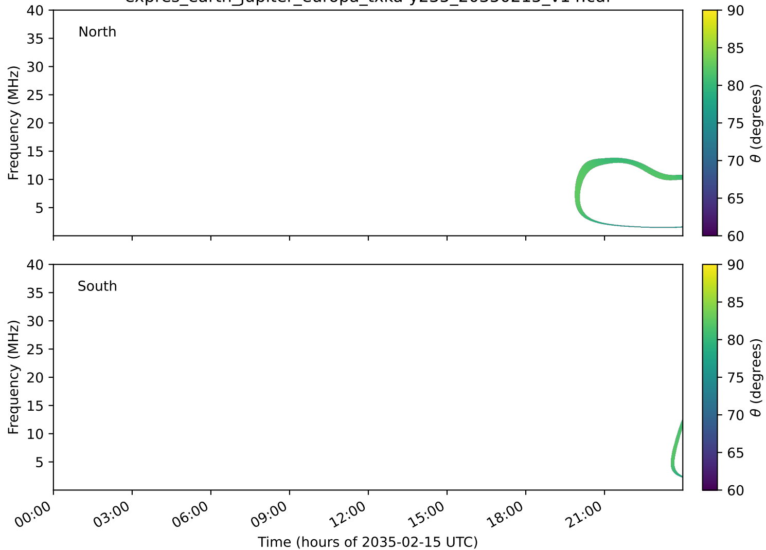
expres_earth_jupiter_europa_txka-y235_20350215_v14.cdf
