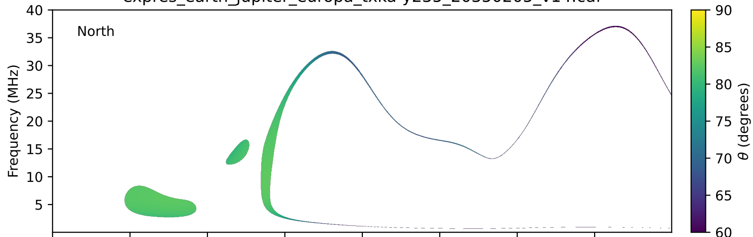
expres_earth_jupiter_europa_txka-y235_20350205_v14.cdf
