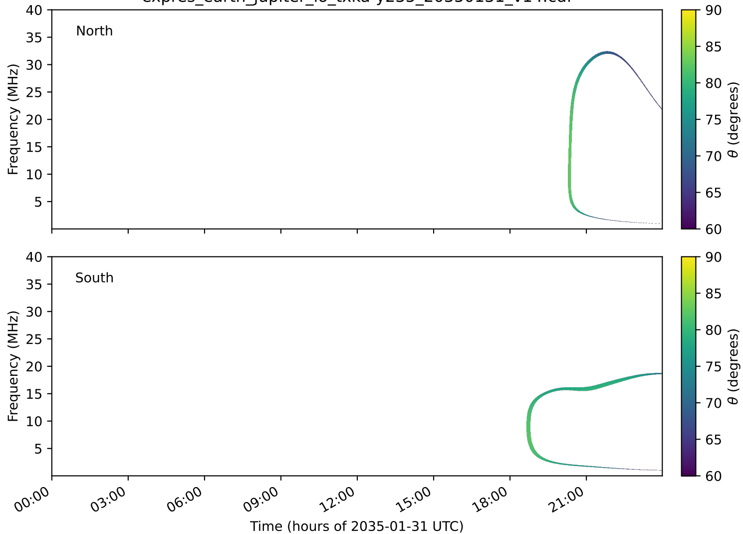
expres_earth_jupiter_io_txka-y235_20350131_v14.cdf
