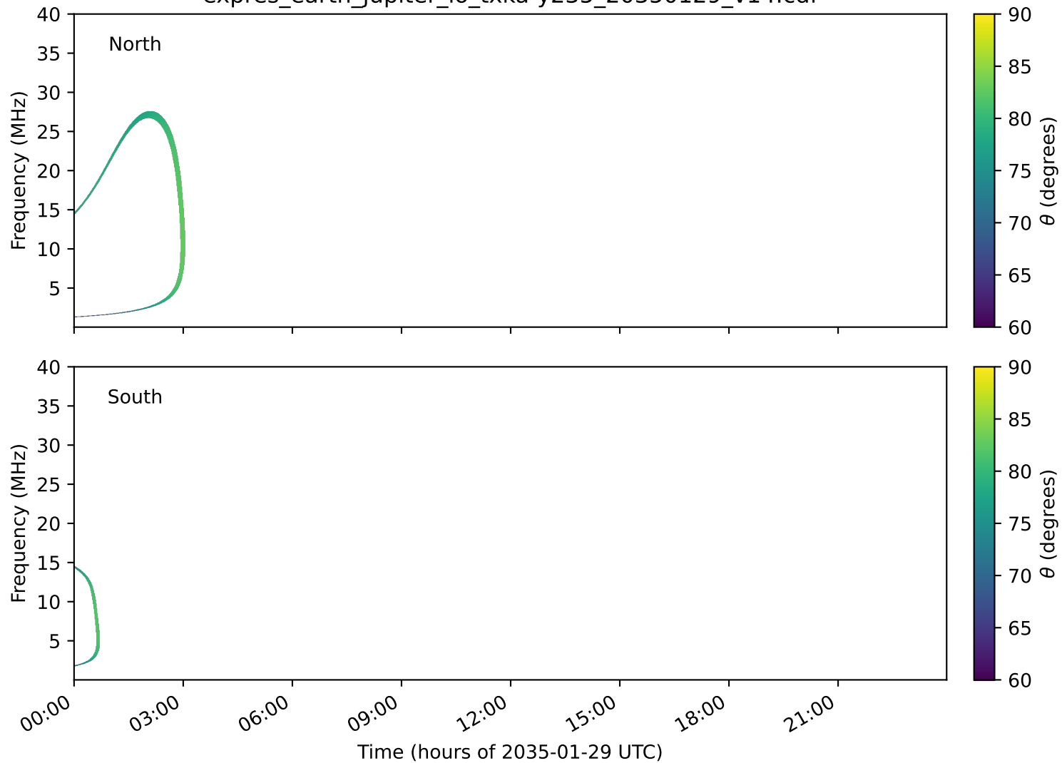
expres_earth_jupiter_io_txka-y235_20350129_v14.cdf
