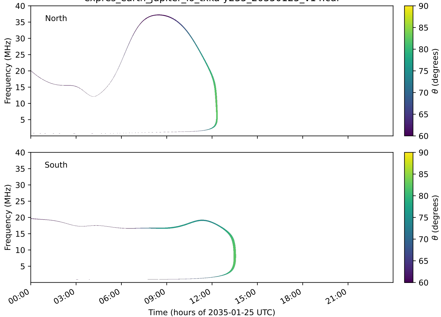
expres_earth_jupiter_io_txka-y235_20350125_v14.cdf
