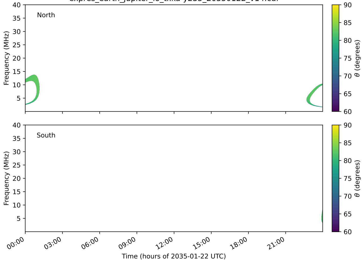
expres_earth_jupiter_io_txka-y235_20350122_v14.cdf
