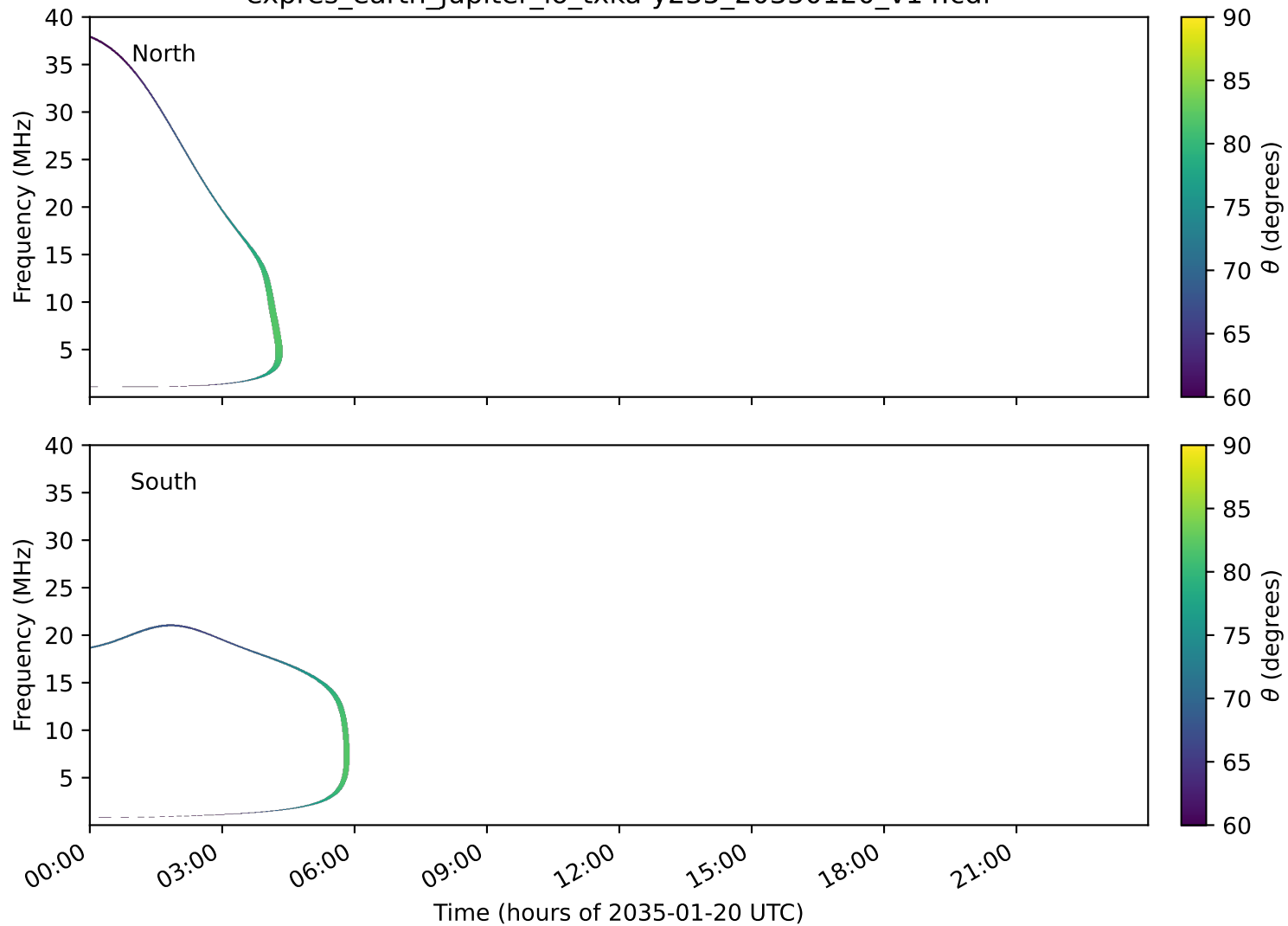
expres_earth_jupiter_io_txka-y235_20350120_v14.cdf
