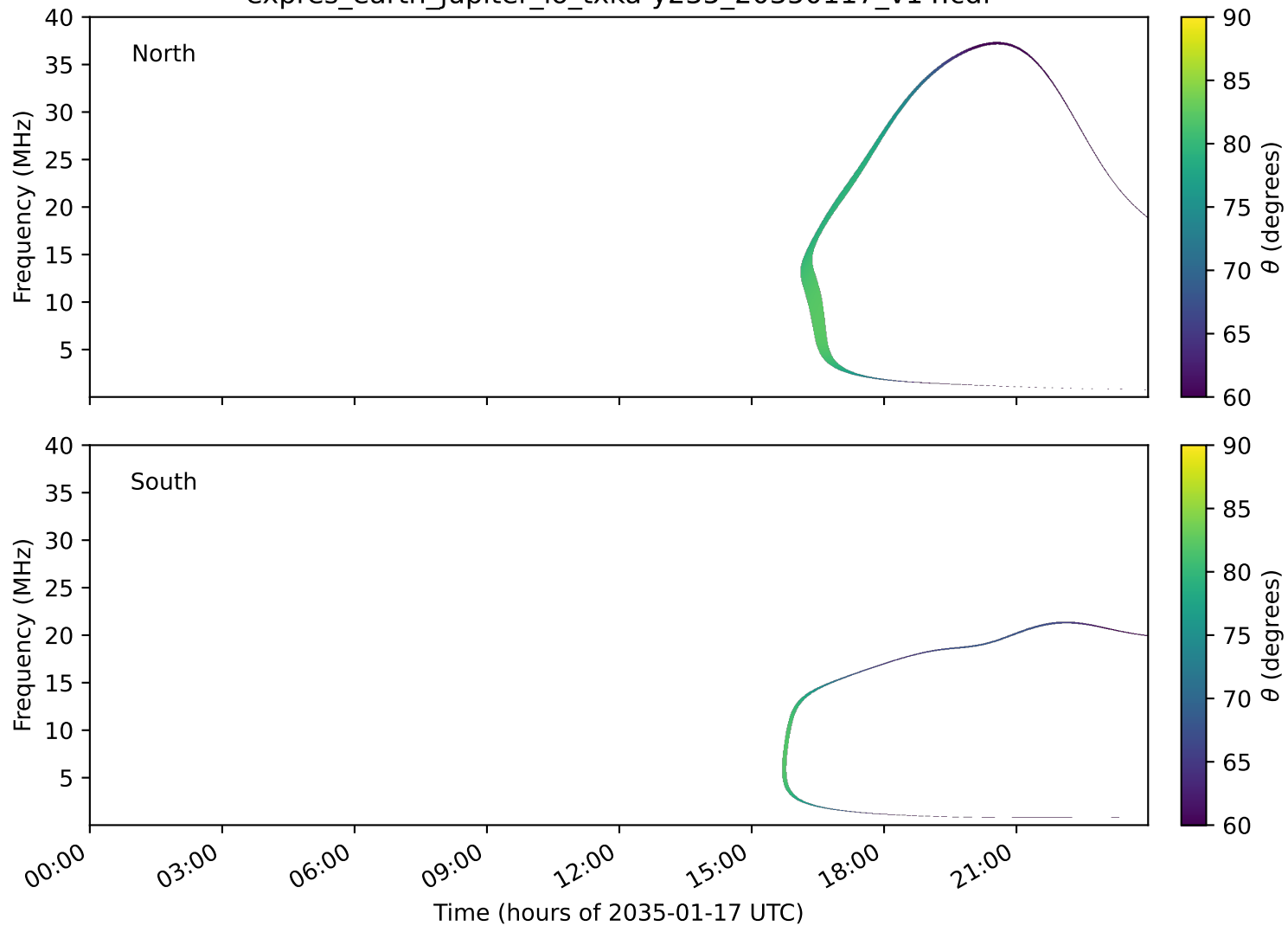
expres_earth_jupiter_io_txka-y235_20350117_v14.cdf
