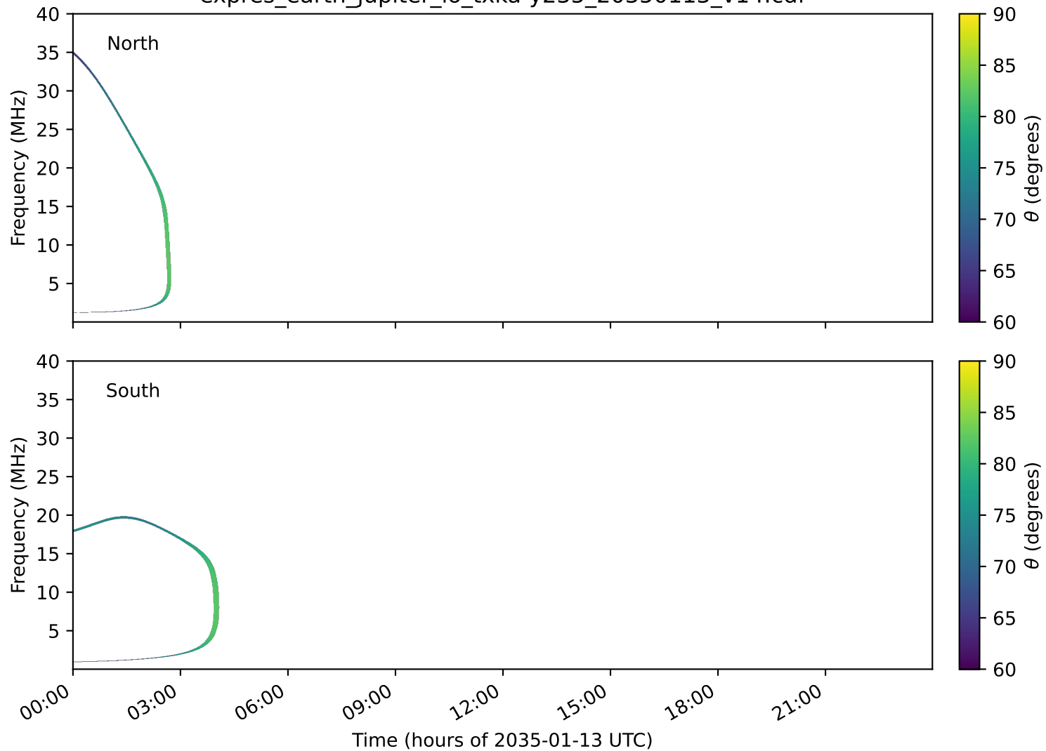
expres_earth_jupiter_io_txka-y235_20350113_v14.cdf
