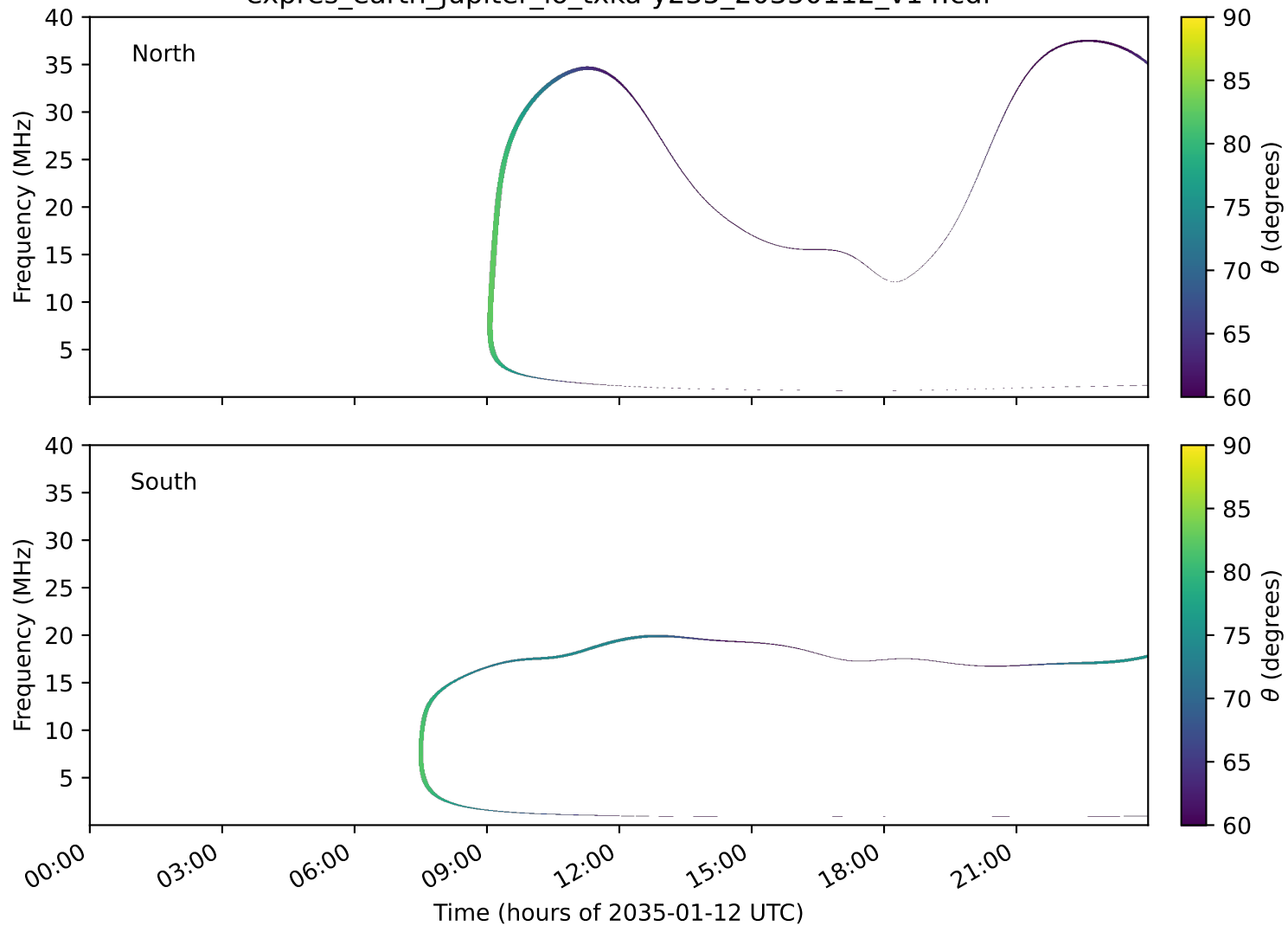
expres_earth_jupiter_io_txka-y235_20350112_v14.cdf
