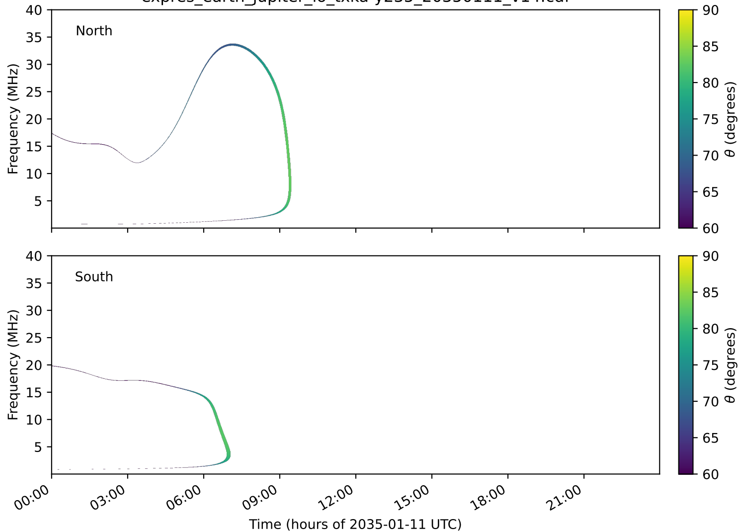
expres_earth_jupiter_io_txka-y235_20350111_v14.cdf
