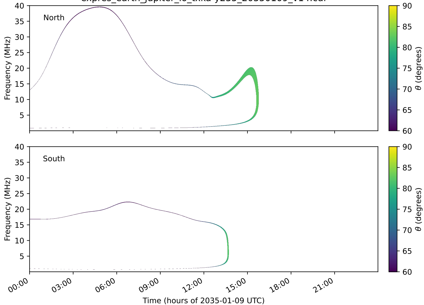
expres_earth_jupiter_io_txka-y235_20350109_v14.cdf
