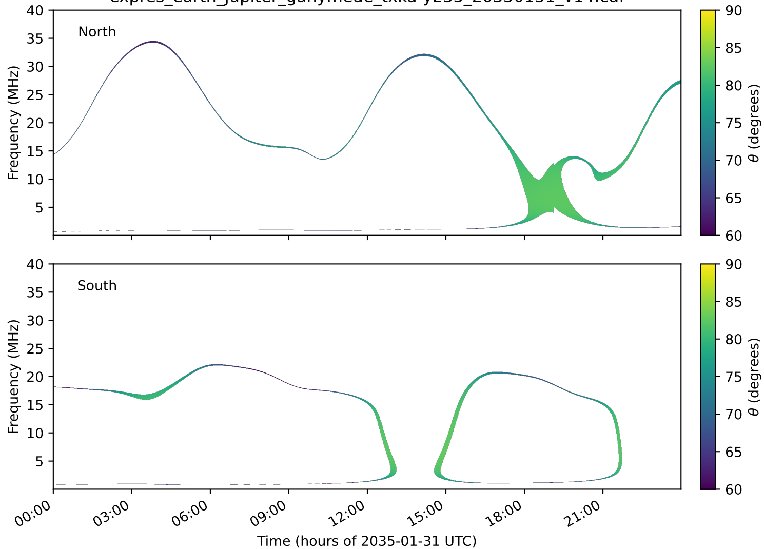
expres_earth_jupiter_ganymede_txka-y235_20350131_v14.cdf
