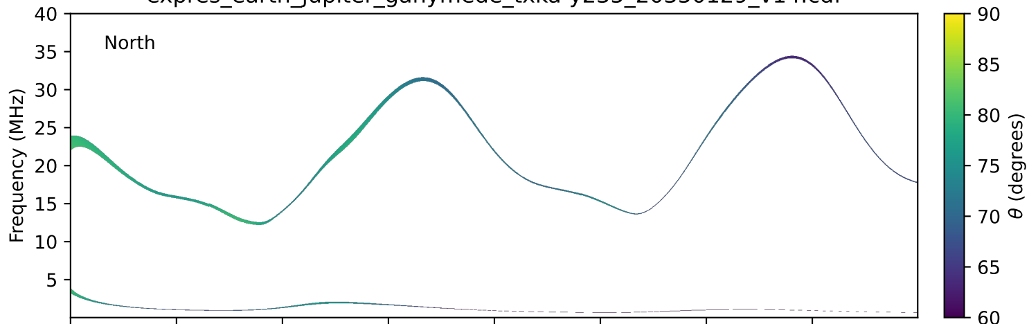
expres_earth_jupiter_ganymede_txka-y235_20350129_v14.cdf
