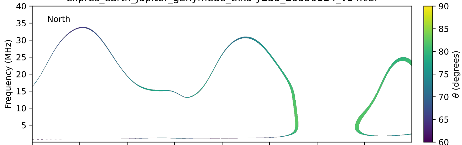
expres_earth_jupiter_ganymede_txka-y235_20350124_v14.cdf
