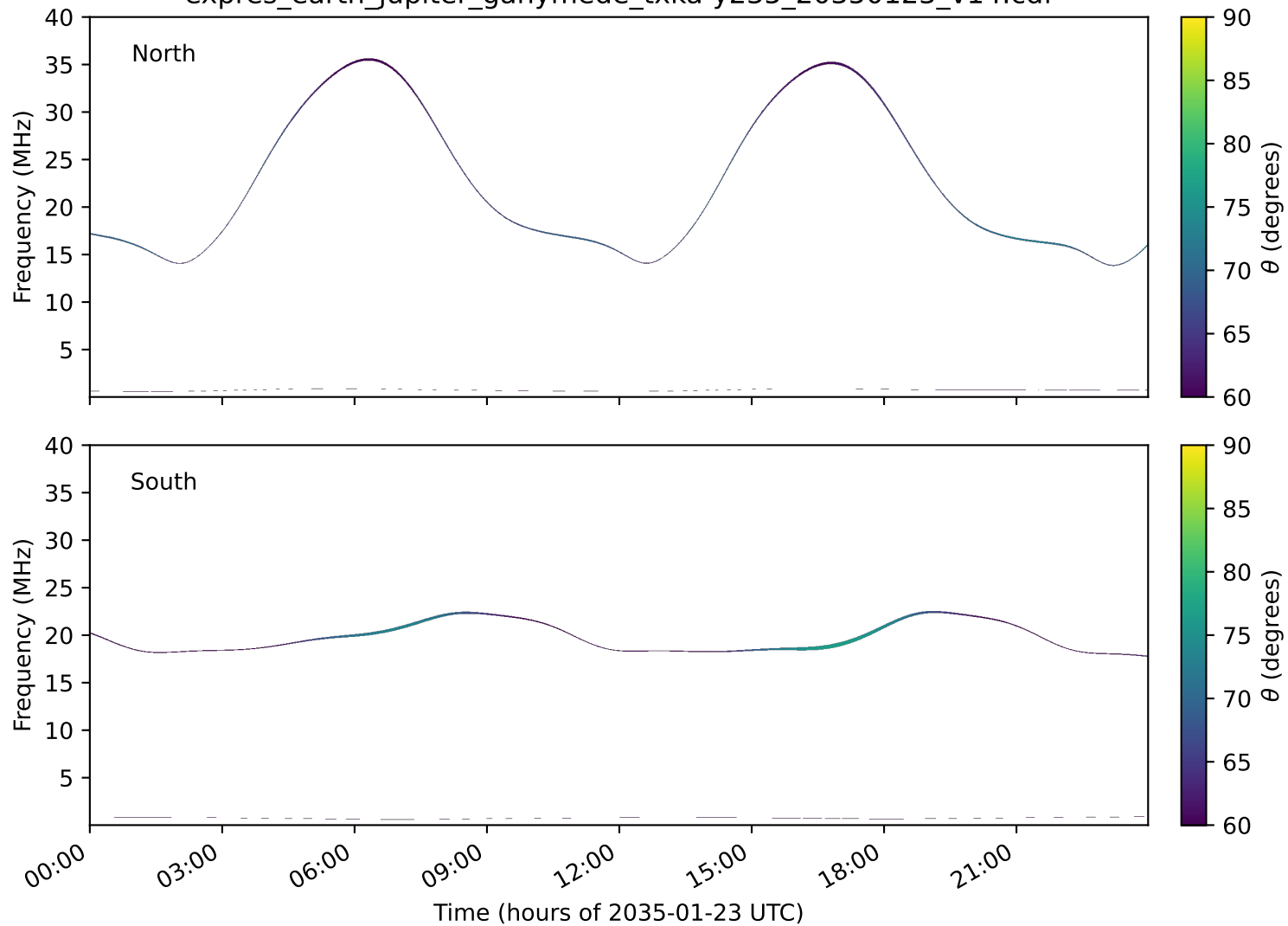
expres_earth_jupiter_ganymede_txka-y235_20350123_v14.cdf
