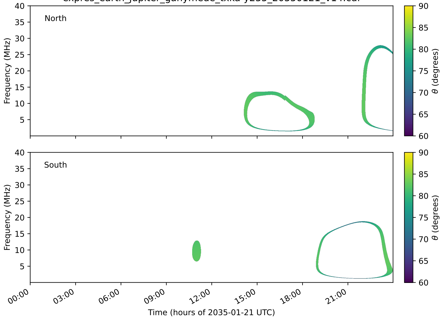
expres_earth_jupiter_ganymede_txka-y235_20350121_v14.cdf
