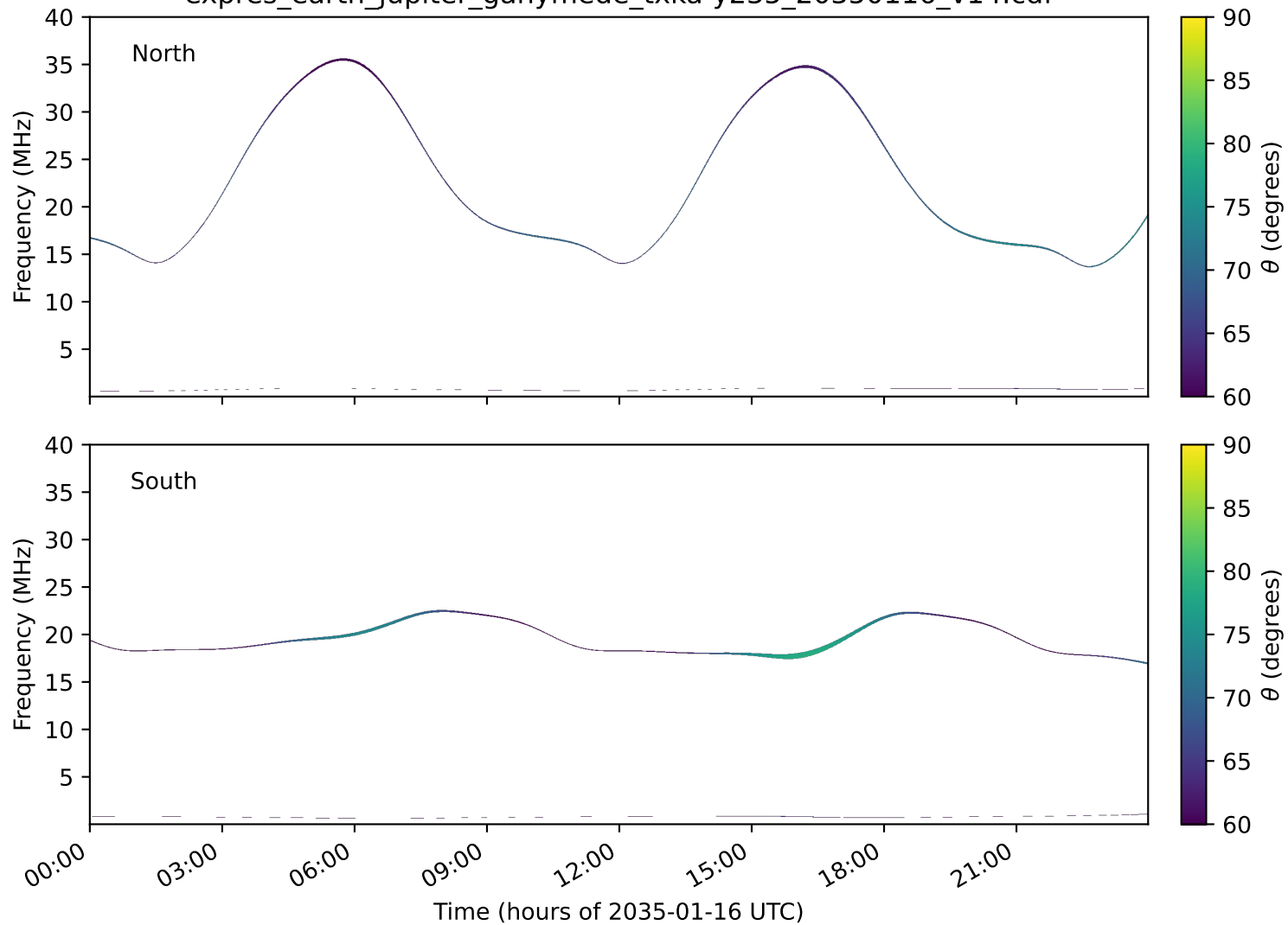
expres_earth_jupiter_ganymede_txka-y235_20350116_v14.cdf
