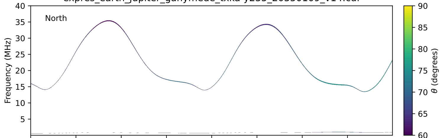
expres_earth_jupiter_ganymede_txka-y235_20350109_v14.cdf
