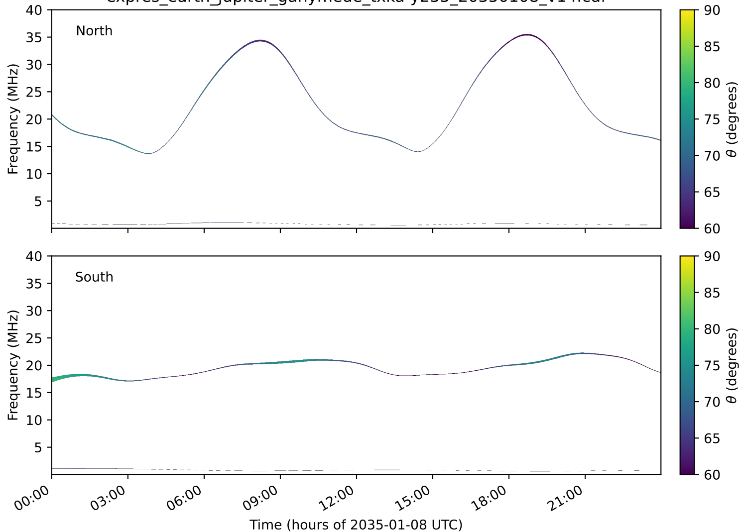
expres_earth_jupiter_ganymede_txka-y235_20350108_v14.cdf
