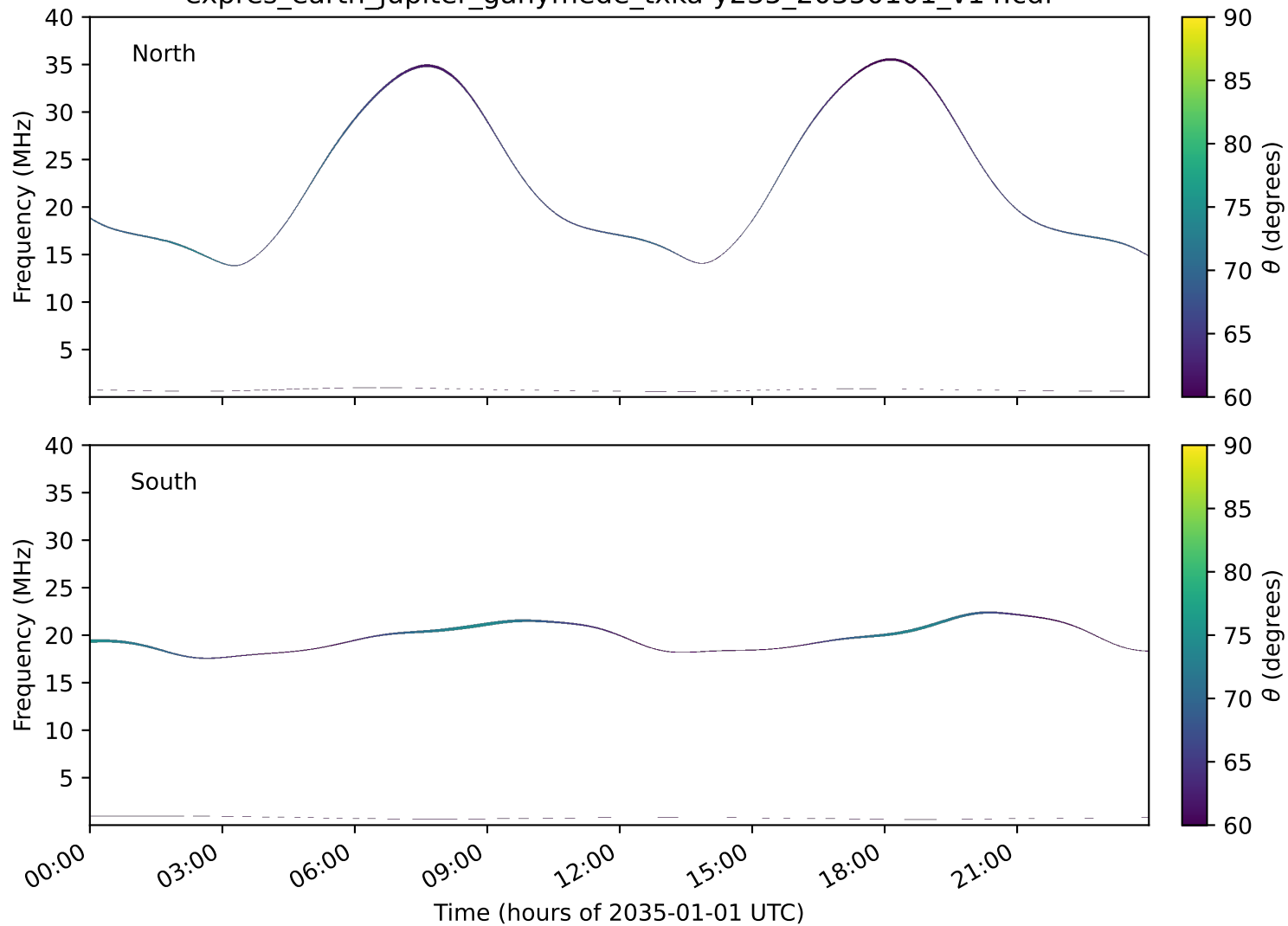
expres_earth_jupiter_ganymede_txka-y235_20350101_v14.cdf
