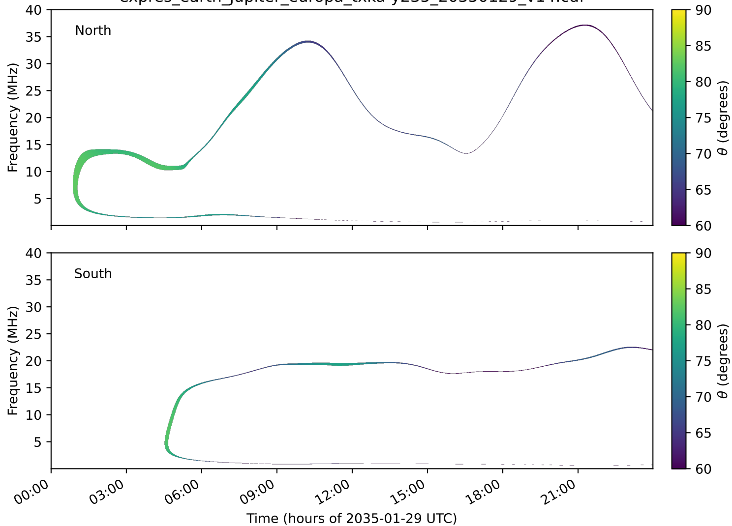
expres_earth_jupiter_europa_txka-y235_20350129_v14.cdf
